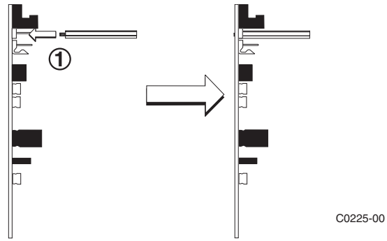
Figure 4a: Installation of IDP-Monitor-10 module in a rear chassis position, method two
