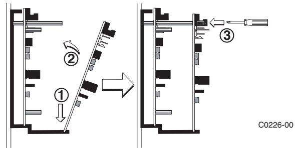
Figure 4b: Installation of IDP-Monitor-10 module in front chassis position
