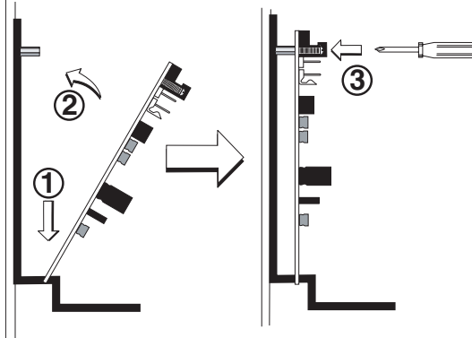
Figure 3: Installation of rear module only, method one
