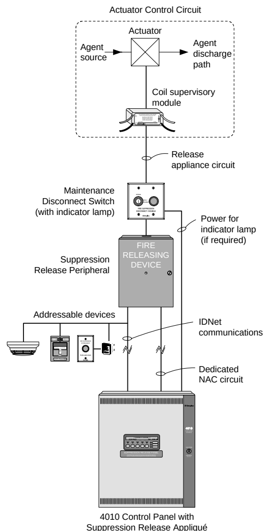
4010 Series Releasing Control Typical Block Diagram
