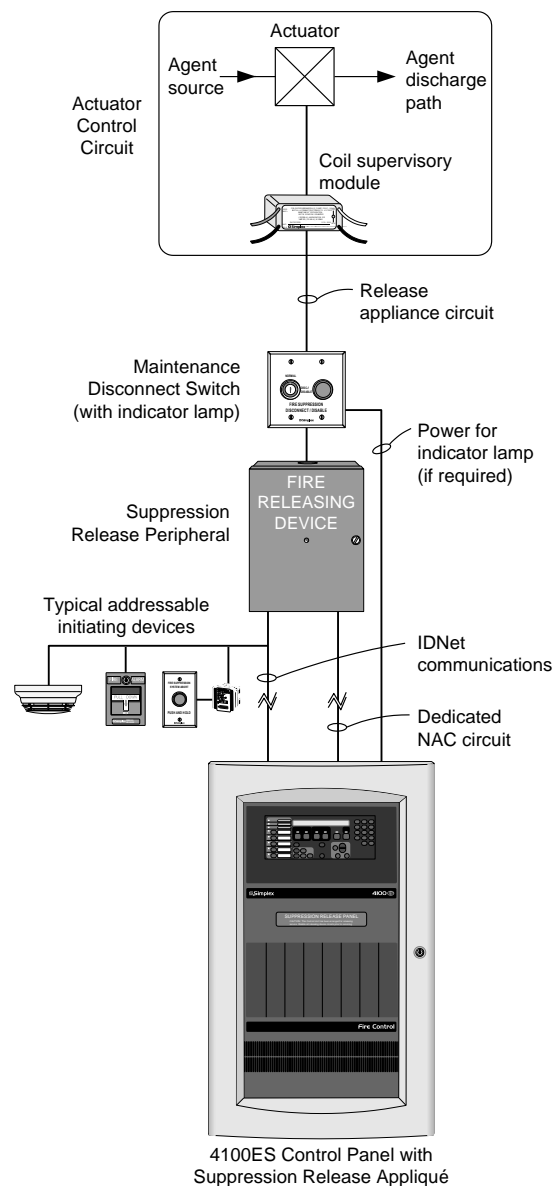
4100ES Series Releasing Control Typical Block Diagram
