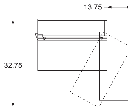
Recommended Clearance Dimensions (Top View)
