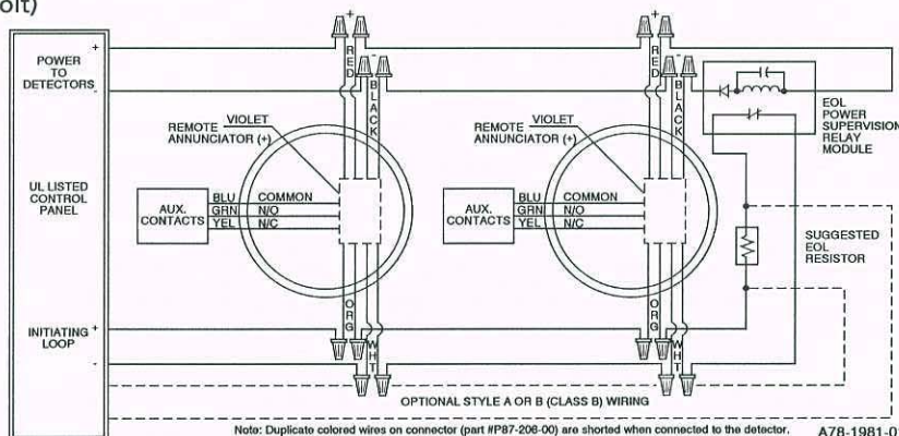
WIRING DIAGRAM FOR 2312/24T DETECTOR
