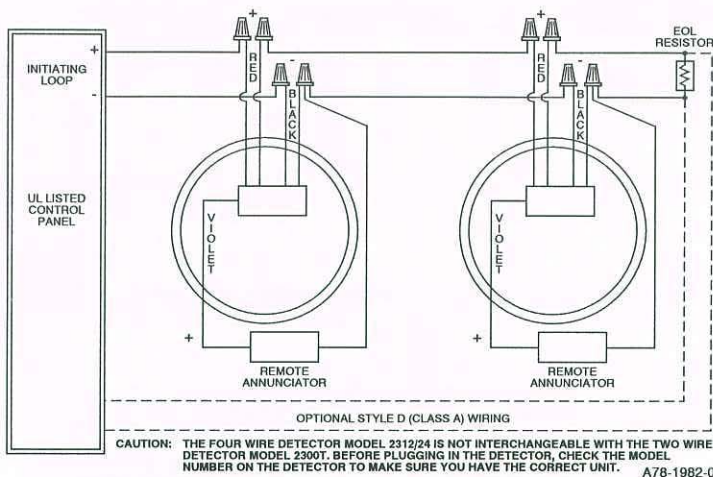
WIRING DIAGRAM FOR 2300T DETECTOR
