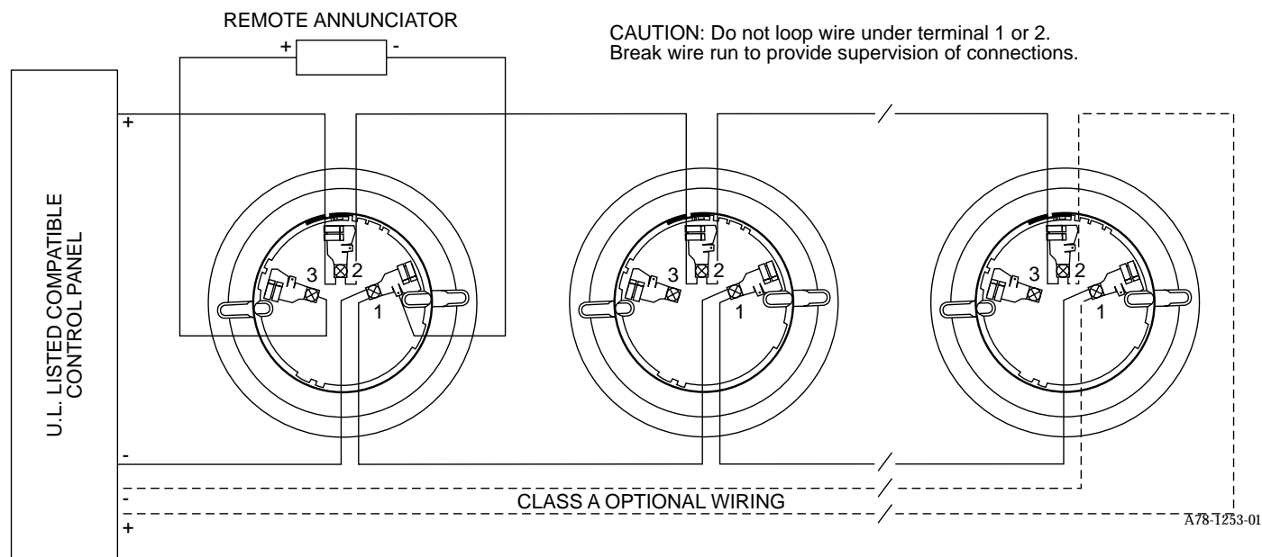
Figure 1. Wiring Diagram:
