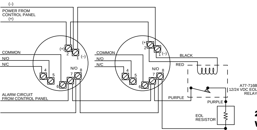
2412B/THB, 2424/TH Wiring Diagram
