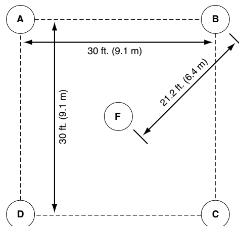
Figure 19: Typical Detector Spacing
